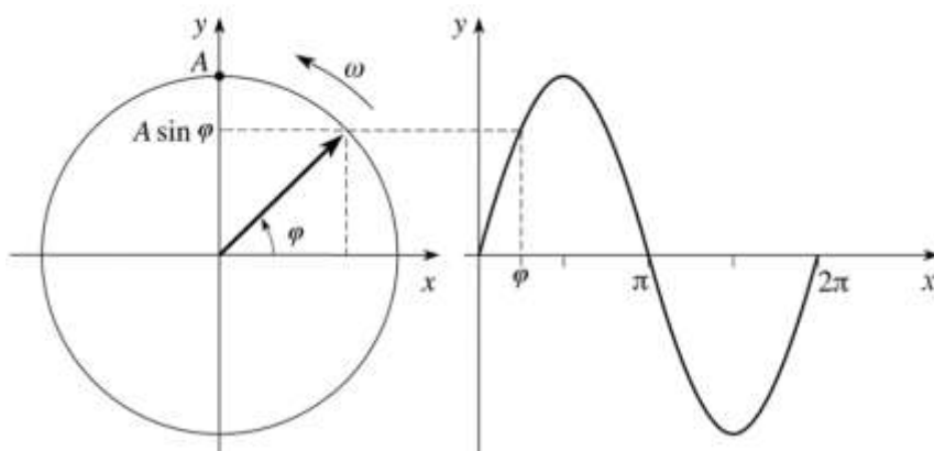
Figure 2: The phasor model allows to visualize the values of the phase and the displacement at any moment. If the angle (i.e. the phase ) of this vector with respect to the +x-axis is \phi_0 at t = 0 , then at time " t " it will be
