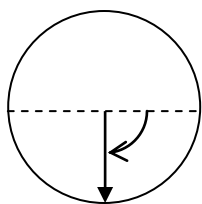
t=0s; \phi=\phi_0=-\pi/2
