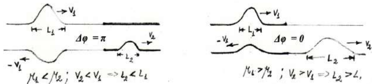
Fig.7 Pulse reflection / transmission through the boundary of two strings with different mass densities
